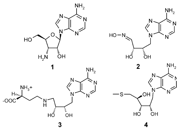
Figure 2. Compounds prepared for this study.
