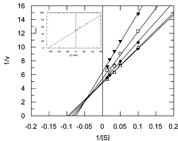
Figure 5. Reversible inactivation of AdoHcy hydrolase with compound 3 . The enzyme was tested in the presence of 0 \mu\text{M} ( \bullet ), 5 \mu\text{M} ( \Delta ), 10 \mu\text{M} ( \blacklozenge ), 25 \mu\text{M} ( \square ) or 50 \mu\text{M} ( \blacktriangledown ) of the compound at 37 °C. Inset: Plot of the slope of the lines as a function of [I] . Data were the average of triplicate measurements. This was reproducible throughout a number of repeated trials.
