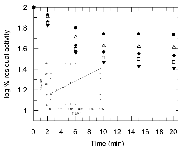
Figure 3. Time-dependent inactivation of AdoHcy hydrolase with compound 1 . The enzyme was preincubated for the indicated times at 37 °C in the presence of 25 \mu\text{M} (●), 50 \mu\text{M} (△), 75 \mu\text{M} (◆), 100 \mu\text{M} (□) or 150 \mu\text{M} (▼) of the compound. At the indicated time points, residual enzyme activity was determined in the hydrolytic direction as stated in the text. Inset: plot of k_{\text{obs}}^{-1} versus [\text{inhibitor}]^{-1} from which the K_i and k_{\text{inact}} values were calculated. The values for compound 1 were determined for time points \leq 6 min. Data were the average of triplicate measurements. This was reproducible throughout a number of repeated trials.
