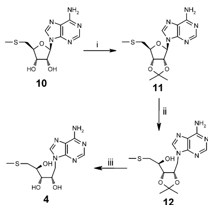
Scheme 2. Synthesis of compound 4 : (i) 2,2-dimethoxypropane, TsOH (ii) DIBAL-H (5 equiv), THF (iii) 8/1 TFA/H 2 O.
