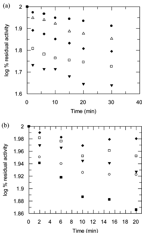
Figure 4. Time-dependent inactivation of AdoHcy hydrolase with (a) compound 2 and (b) compound 4 . The enzyme was preincubated for the indicated times at 37 °C in the presence of 5 \mu\text{M} ( \bullet ), 10 \mu\text{M} ( \Delta ), 25 \mu\text{M} ( \blacklozenge ), 50 \mu\text{M} ( \square ), 75 \mu\text{M} ( \blacktriangledown ), 100 \mu\text{M} ( \circ ), or 150 \mu\text{M} ( \blacksquare ) of the appropriate compound. At the indicated time points, residual enzyme activity was determined in the hydrolytic direction as stated in the text. Data were the average of triplicate measurements. This was reproducible throughout a number of repeated trials.
