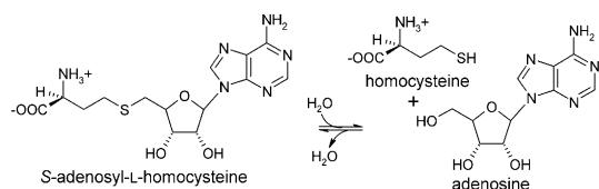
Figure 1. Reaction catalyzed by S -adenosyl-L-homocysteine hydrolase.
