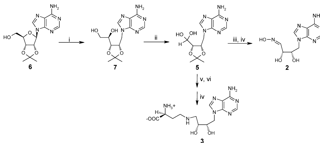
Scheme 1. The synthesis of compounds 2 and 3 : (i) DIBAL-H (5 equiv), THF (ii) NaIO 4 , H 2 O (iii) NH 2 OH-HCl, NaOMe, MeOH (iv) 8:1 TFA/H 2 O (v) N -Boc-L-,2-diaminobutyric acid, MeOH (vi) NaCNBH 4 .
